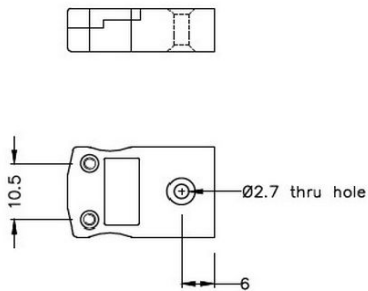
Miniature in-line Socket (dimensions in mm)
